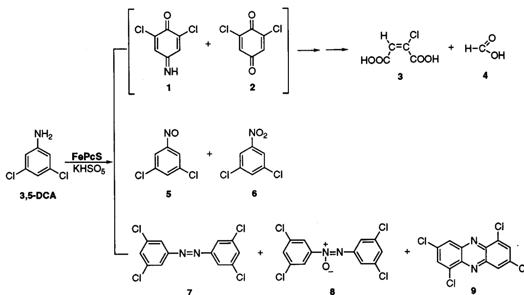
Figure 1. Products formed in the oxidation of 3,5-DCA by FePcS/KHSO 5
